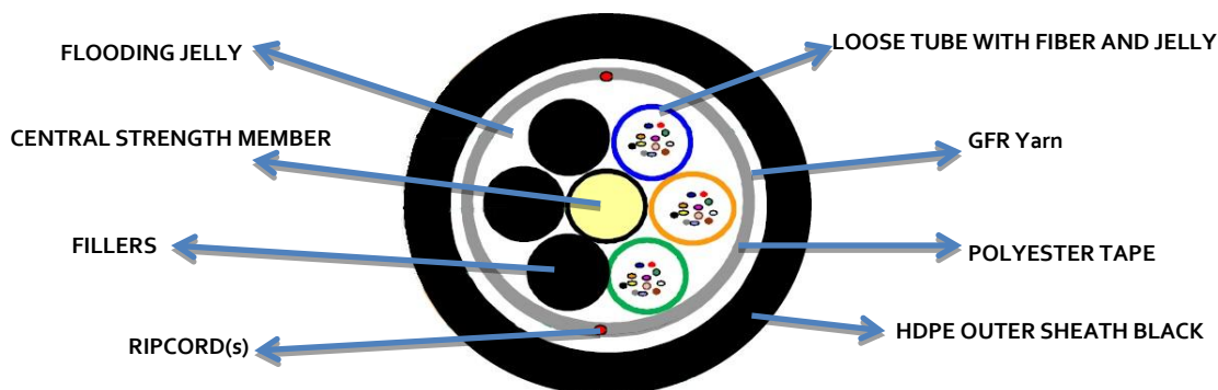
Typical Construction Diagram : Not to the scale
